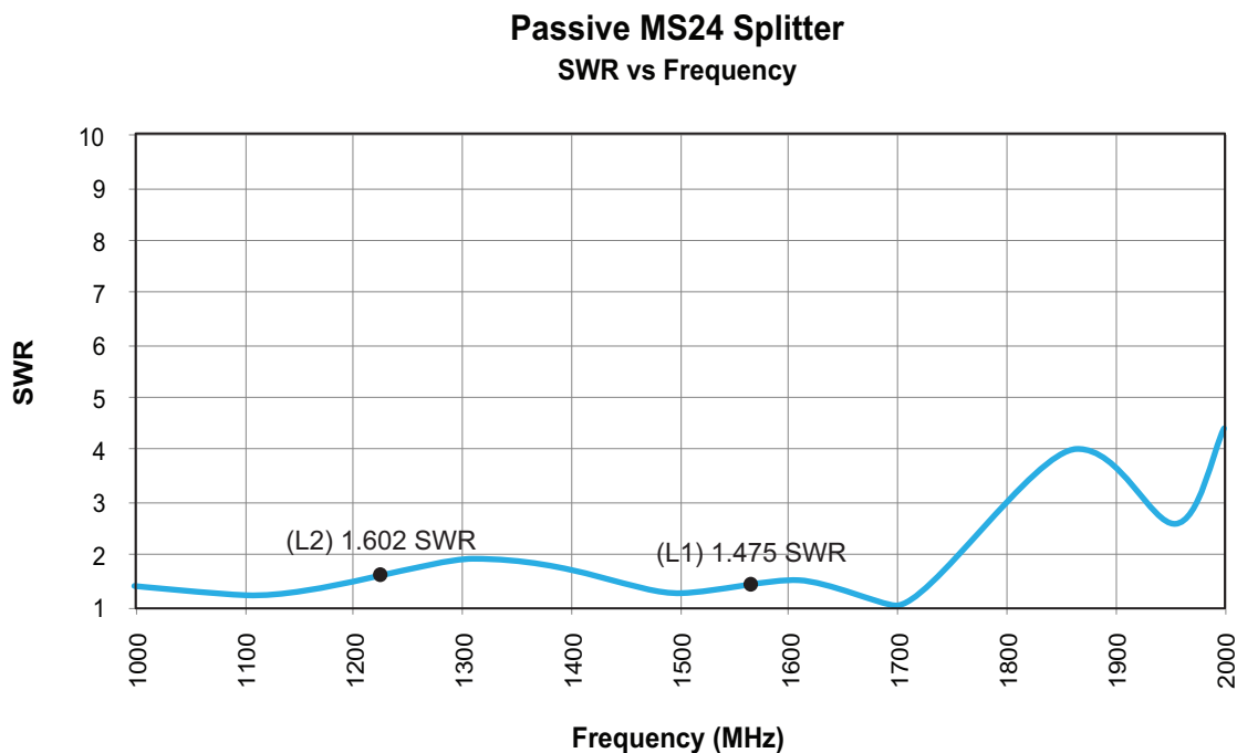
Figure 2-2. Passive MS24 Splitter: Input SWR vs. Frequency
