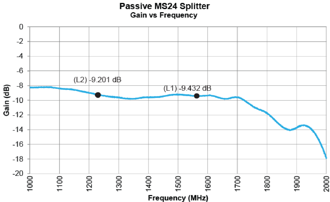
Figure 2-1. Passive MS24 Splitter: Gain vs. Frequency
